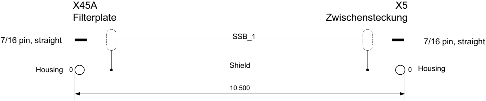
Cable Type: Flexline 7/8"
